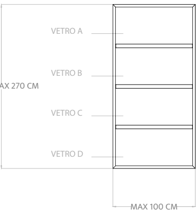
PANNELLO M / M Panel
