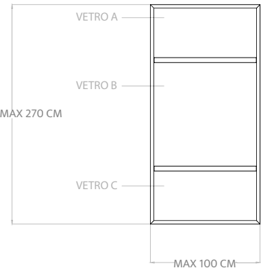
PANNELLO Z / Z Panel
