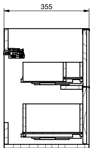
B-B (1:7)
